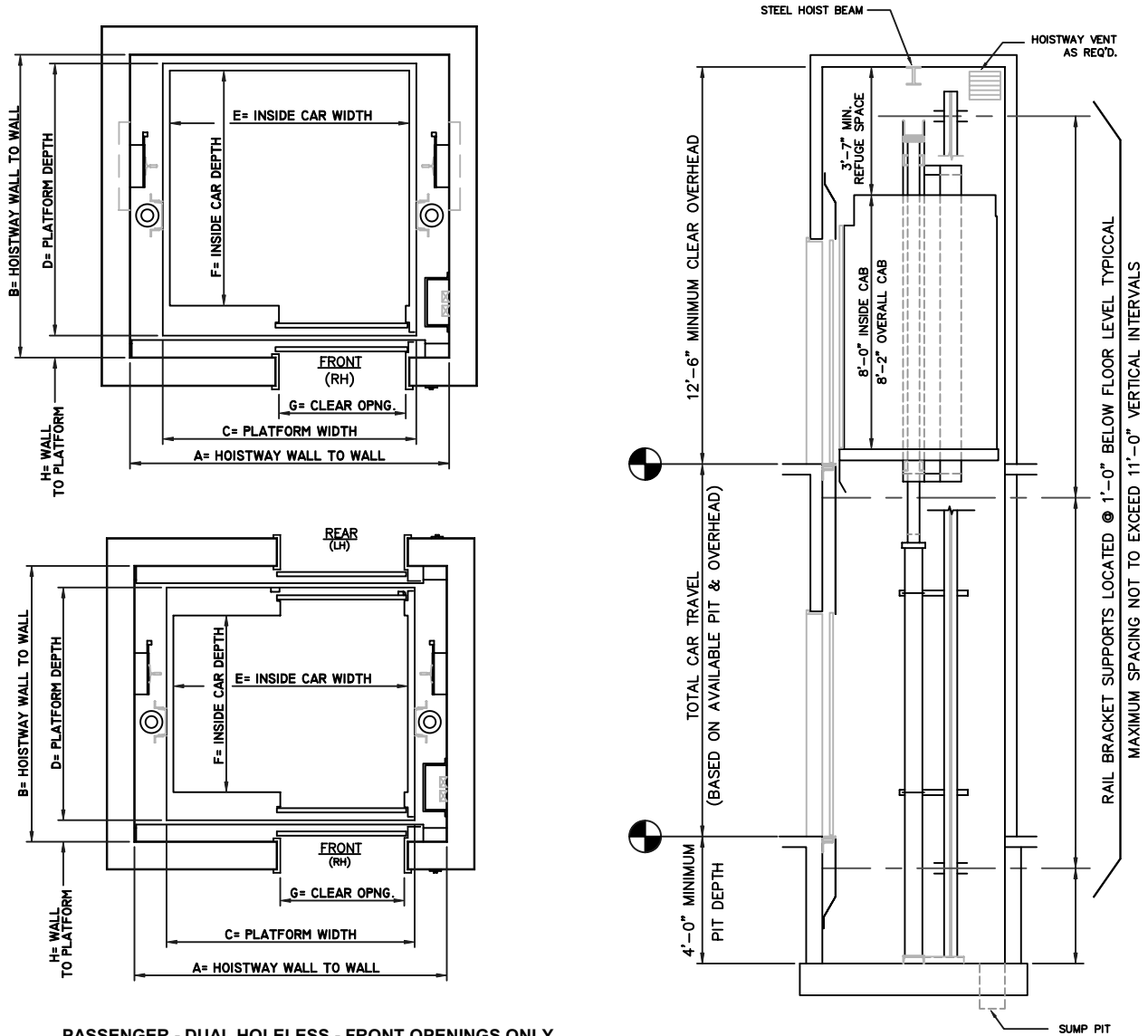
PASSENGER - DUAL HOLELESS - FRONT OPENINGS ONLY
